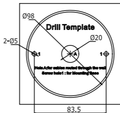
Figure 2-10 The Drill Template
