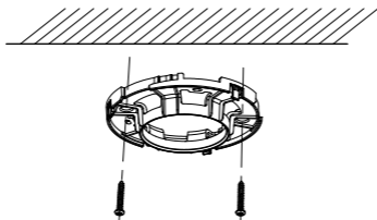
Figure 2-19 Install the Mounting Base
