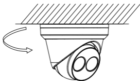
Figure 2-29 Install Trim Ring
