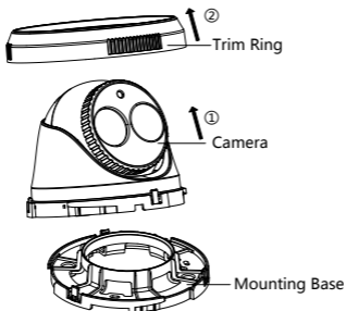
Figure 2-9 Disassemble the Camera
