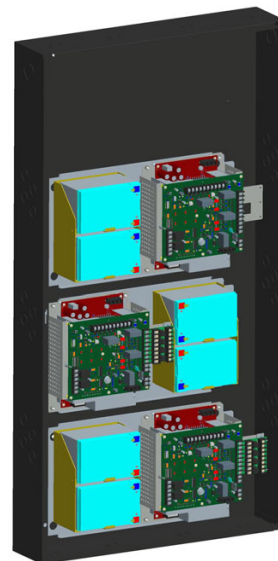
HPFF12CM: Three modules in EQBB-D4
