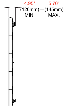
SIDE VIEW WITH MODULES
