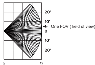
Sensor Optical View (top view, in feet)
