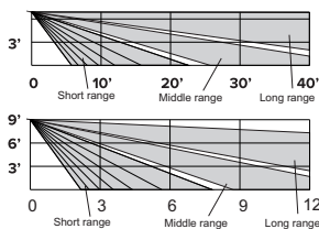
Sensor Optical View Pattern (side view, in feet)
