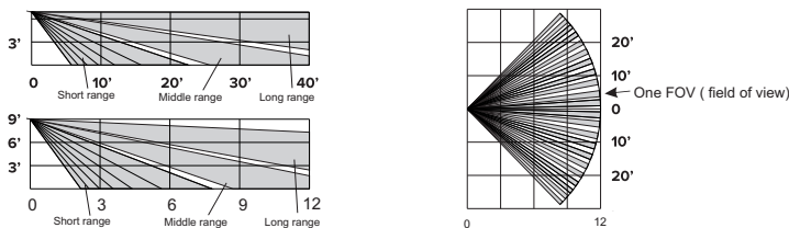
Optical Fields-of-View Long-range (44) Mid-range (36) Short-range (18)
