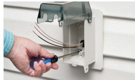
3 Attach box to substrate with screws. Caulk as required.
