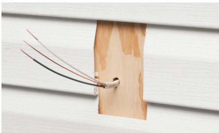
1 Disconnect electrical power. Cut hole in siding.
