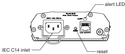
IEC C14 inlet
