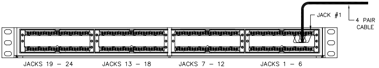
REAR VIEW ANGLED 24 PORT
