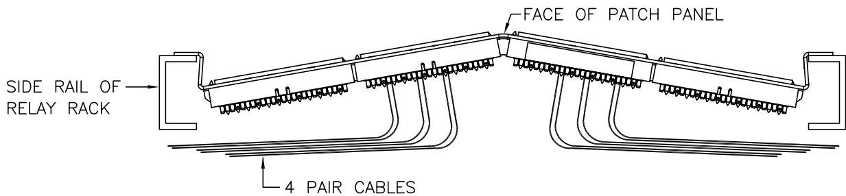
TOP VIEW (SIMPLIFIED)
