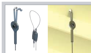
Speed Link SLK with Decking Hook
