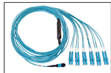
FP3LDMF002M, FX Hydra Patch Cord, OM3, MPO-12F (F) to 6 x LC Duplex, 2 m
