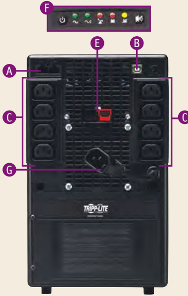
OMNIVSINT1500XL Rear Panel
