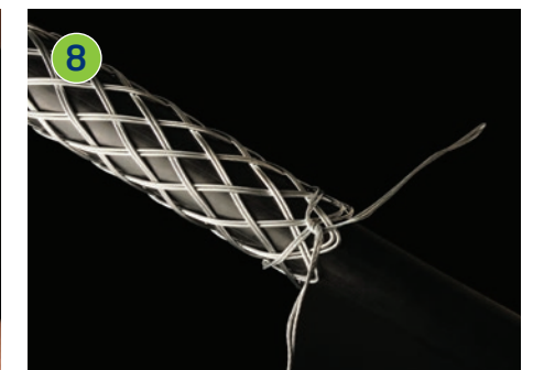
8 Add any additional support as required - banding is recommended. The cable grip is now ready to use.
