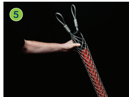
5 The grip then needs to be pushed along so that all the lattice is in contact with the conductor.
