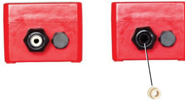
Figure 2. Cable gland with and without the cable entry insert
