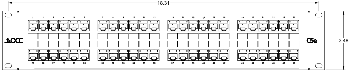
FRONT VIEW (48 PORT)
