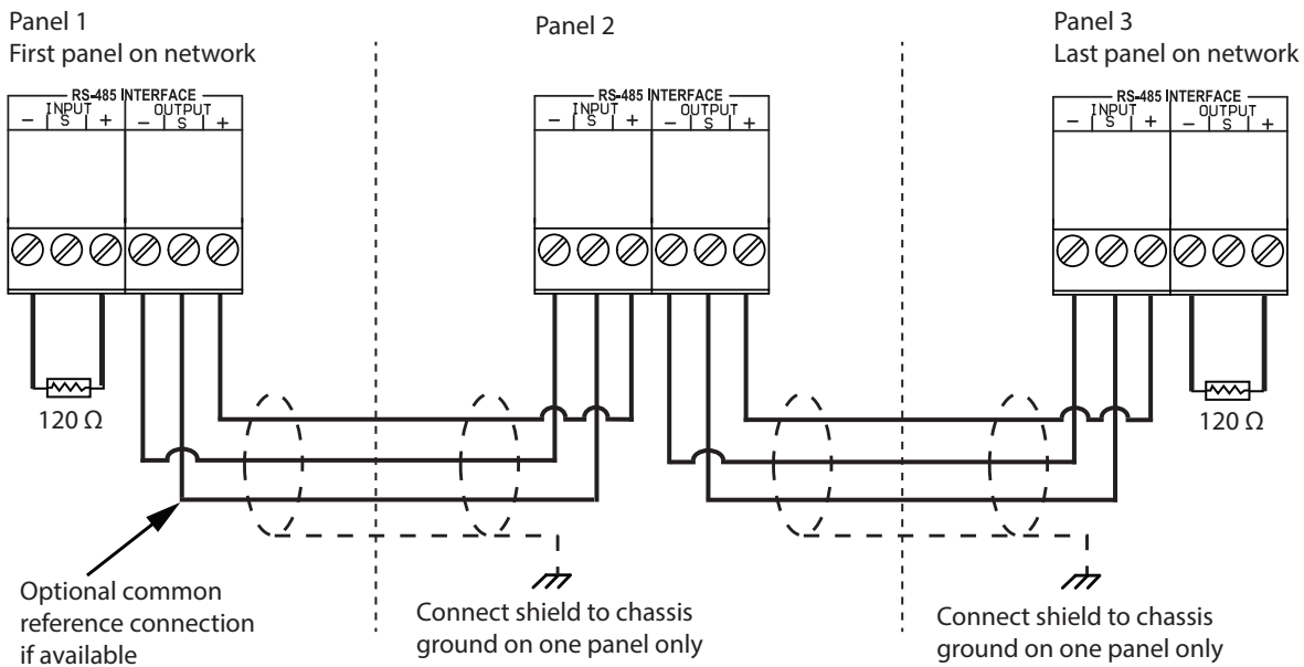
Figure 31. RS-485 Wiring
