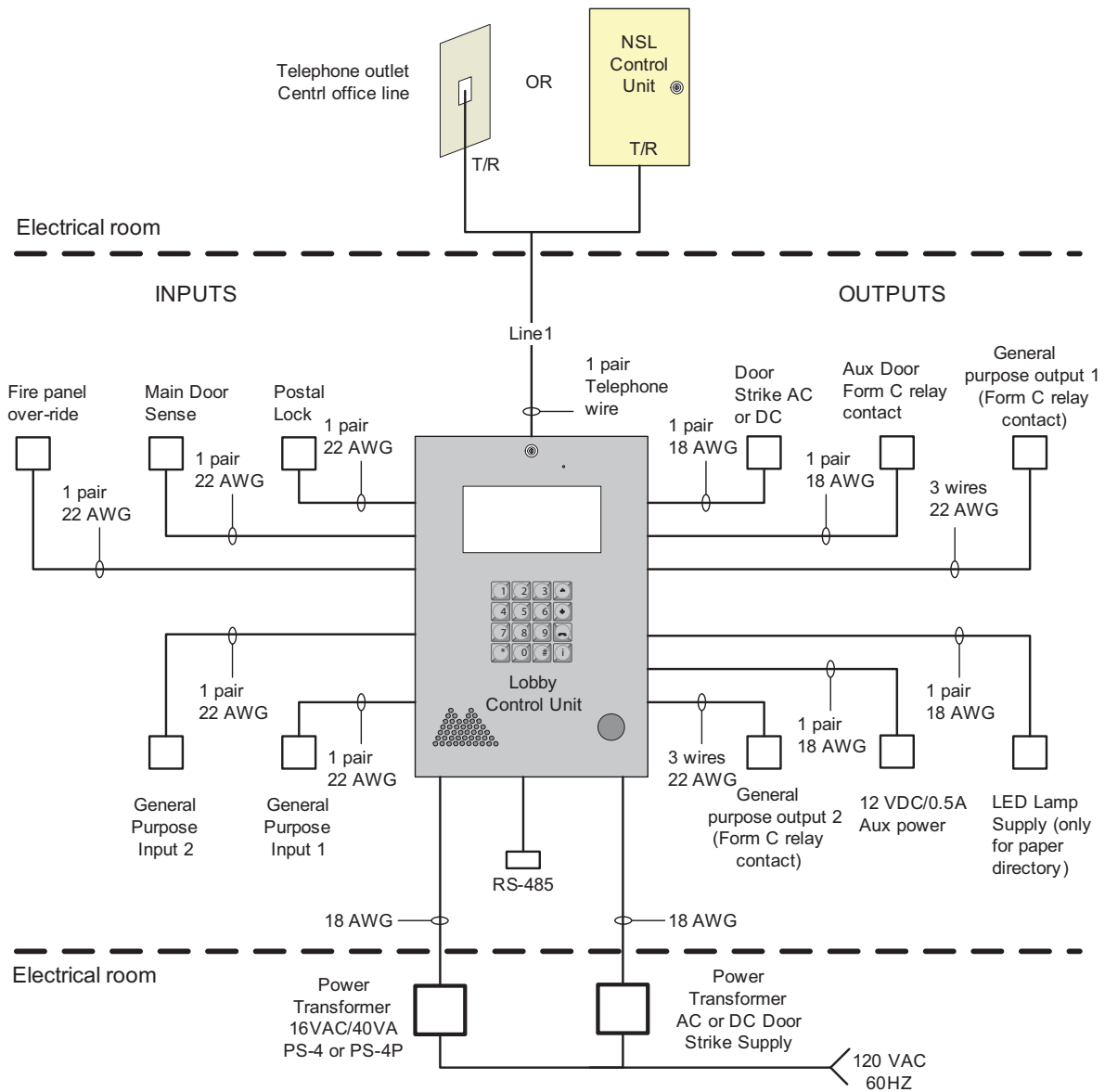
Figure 20. Single Entrance System Wiring
