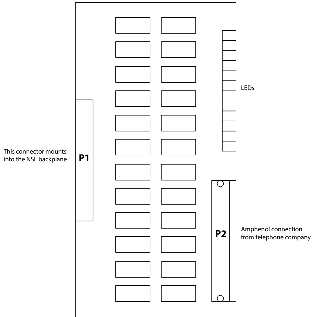
Figure 48. 2012 NSL Relay Board
