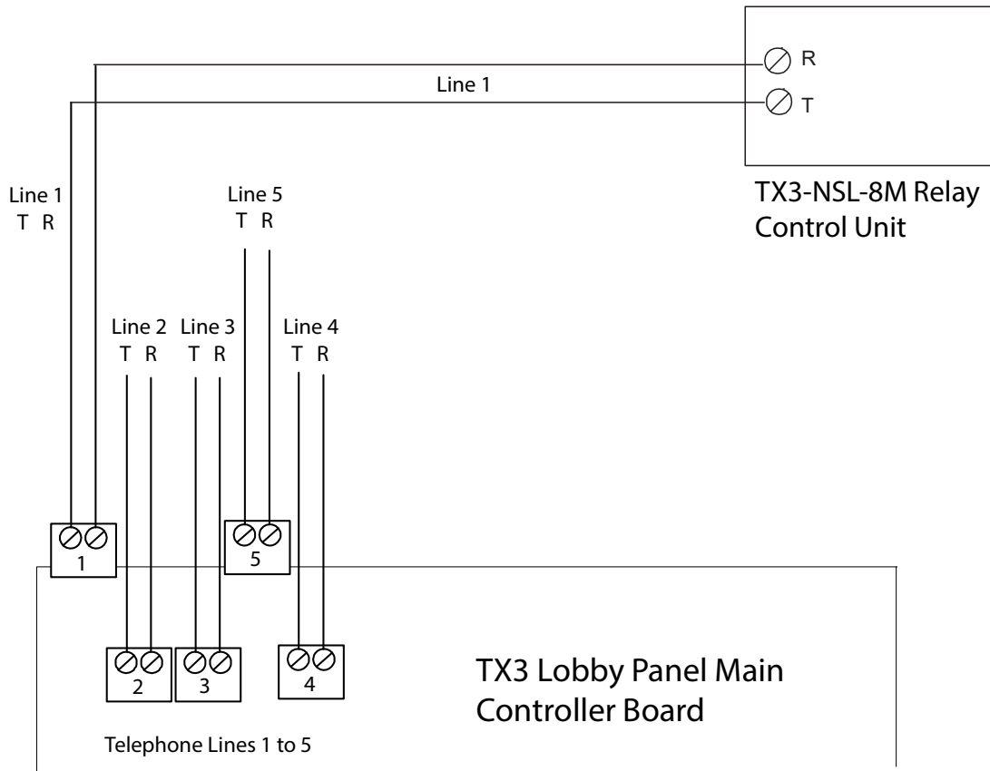
Figure 44. NSL Controller Telephone Lines
