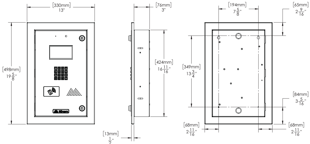
Figure 15 Dimensions of TX3-2000-8CR-C
