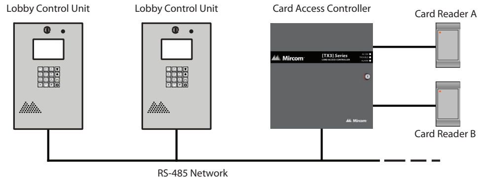
Figure 24. TX3 devices on an RS-485 network.
