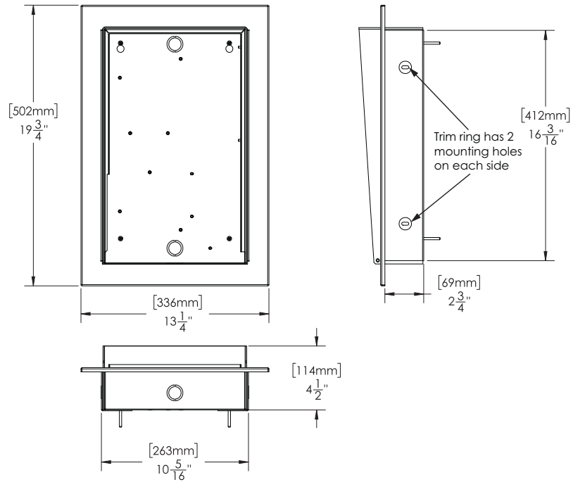
Figure 2 Dimensions of TX3-UFT and the Universal Enclosure
