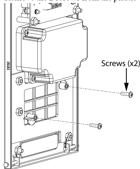
Figure 51. Remove the 2 screws
