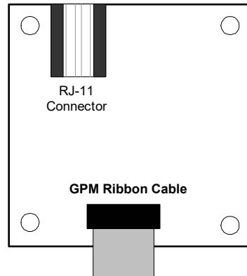
Figure 38. Guard Phone Module
