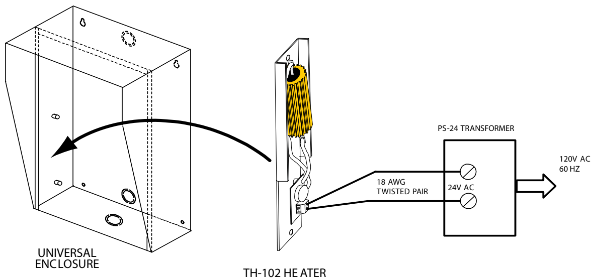
Figure 17 Heater TH-102 Installation Location
