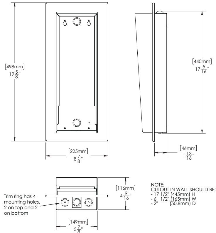
Figure 11 Dimensions of TX3-2000-4UR-C with TX3-USFTR
