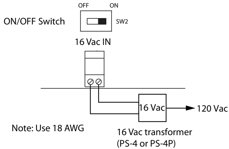
Figure 32. Power Supply
