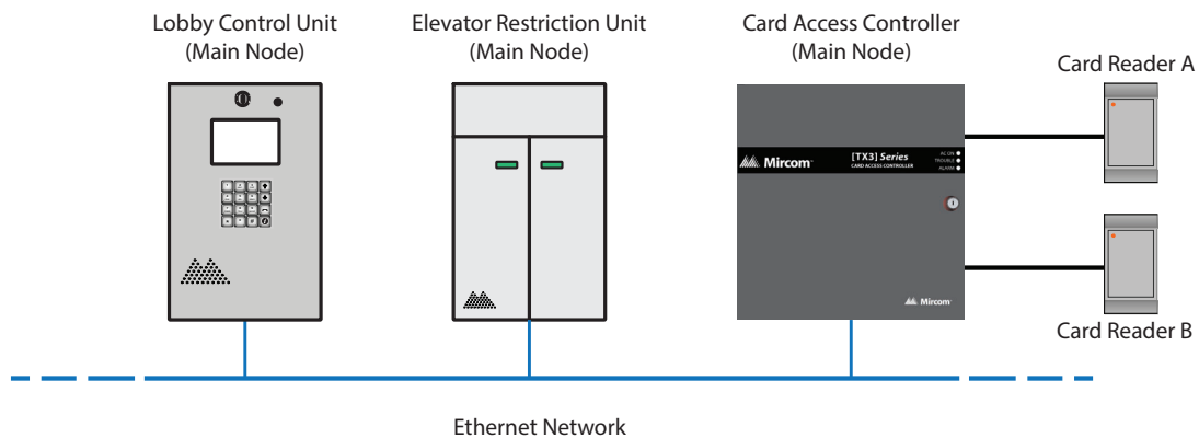
Figure 25. TX3 devices on an Ethernet TCP/IP network.
