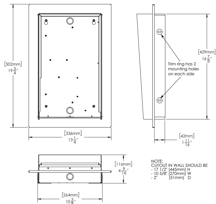
Figure 5 Dimensions of TX3-2000-8UR-C with TX3-UFTR
