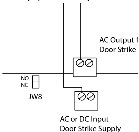
Figure 34. Main Door Dry Contact Wiring
