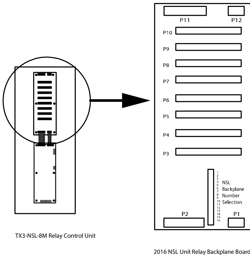
Figure 45. NSL Backplane
