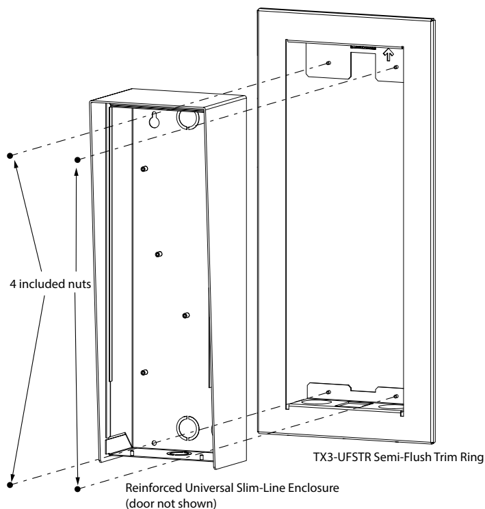
Figure 12 Mount TX3-USFTR Semi-Flush Trim Ring for Reinforced Universal Slim Line Enclosures (door not shown)
