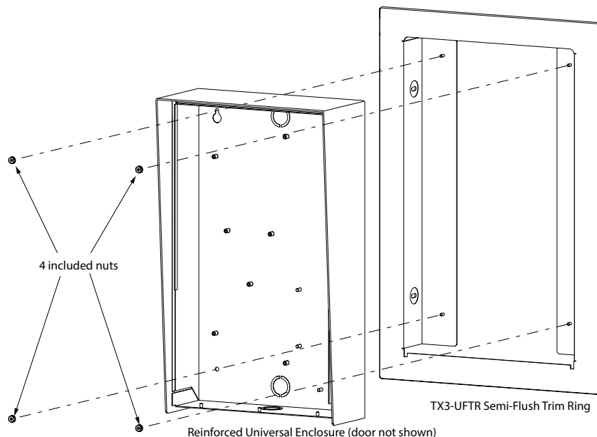
Figure 6 Mount TX3-2000-8UR-C into TX3-UFTR
