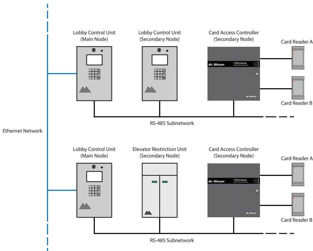
Figure 26. Lobby control units using both Ethernet and RS-485 networks
