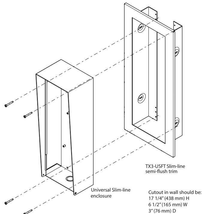
Figure 9 Mount TX3-USFT Universal Slim Line Flush Trim Ring
