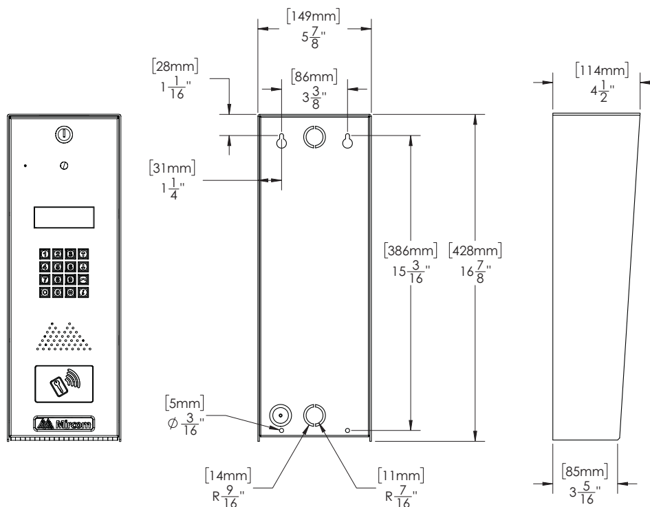
Figure 10 Dimensions of TX3-2000-4UR-C
