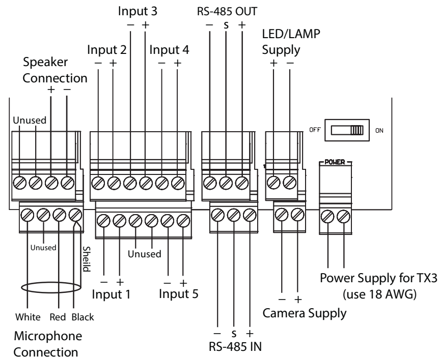
Figure 29. Controller Board Connectors - Bottom
