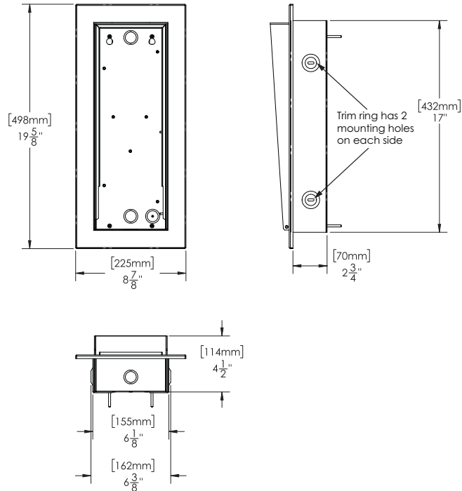
Figure 8 Dimensions of TX3-USFT and the Universal Slim Line Enclosure
