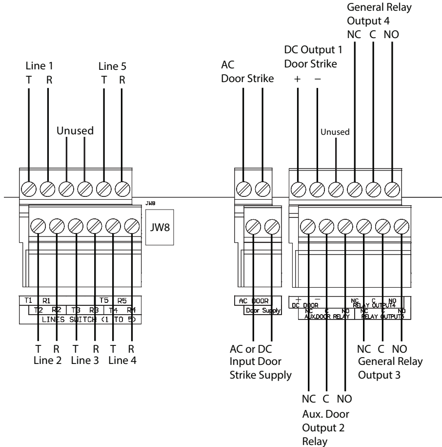
Figure 33. Controller Board Connectors - Top
