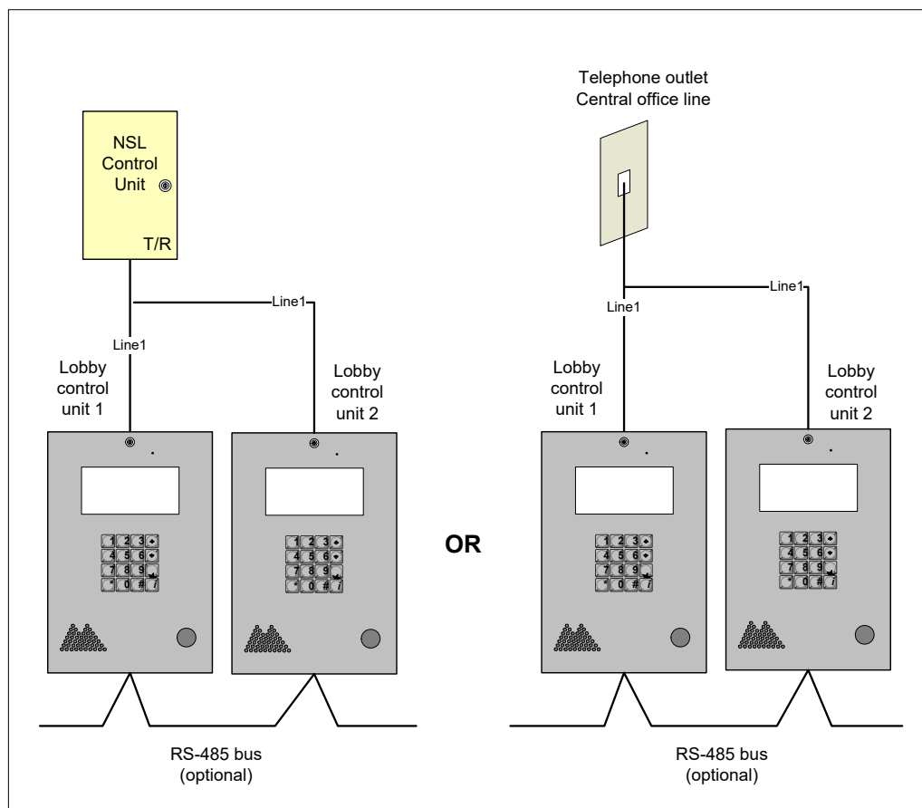
Figure 21. Dual Lobby Control Units
