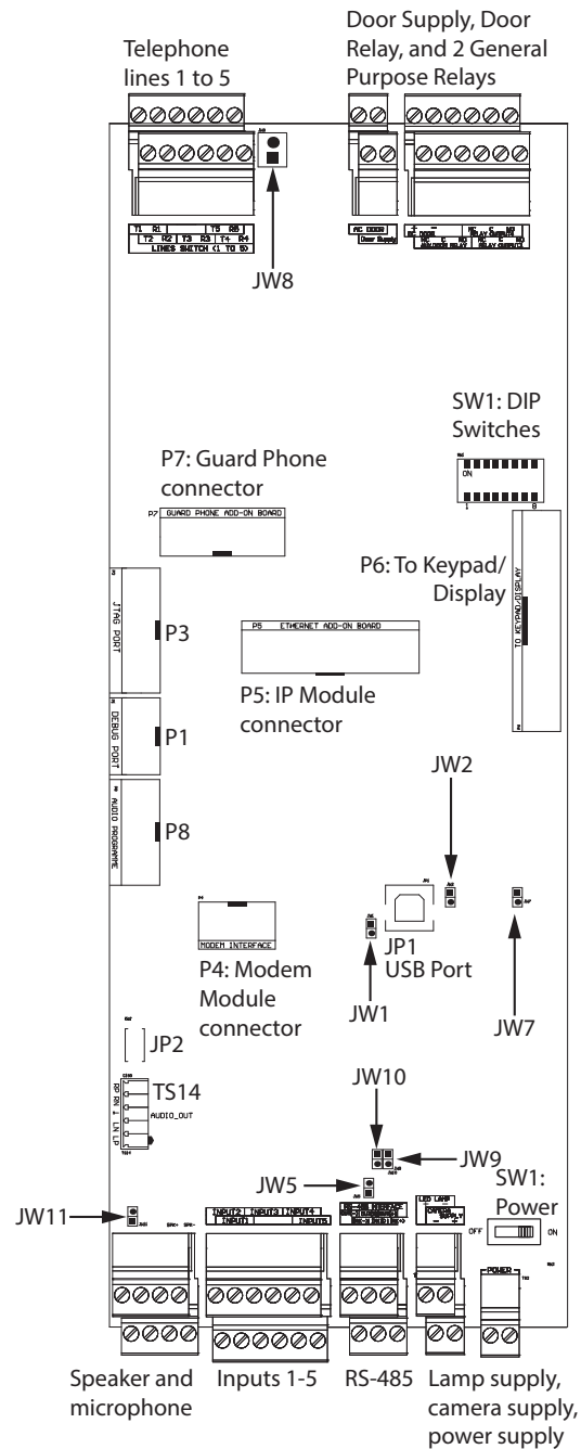
Figure 28. Lobby Control Unit Main Controller Board
