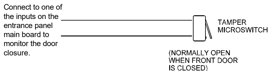
Figure 30. Tamper Switch
