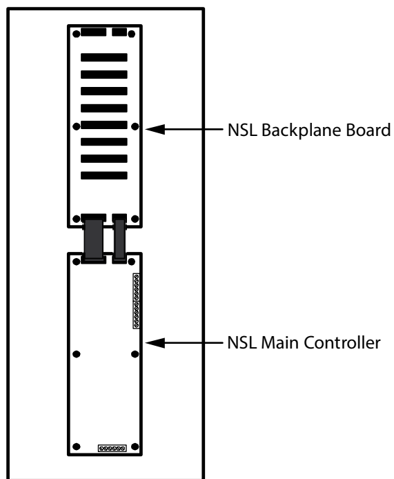
Figure 40. TX3-NSL-8M Relay Control Unit
