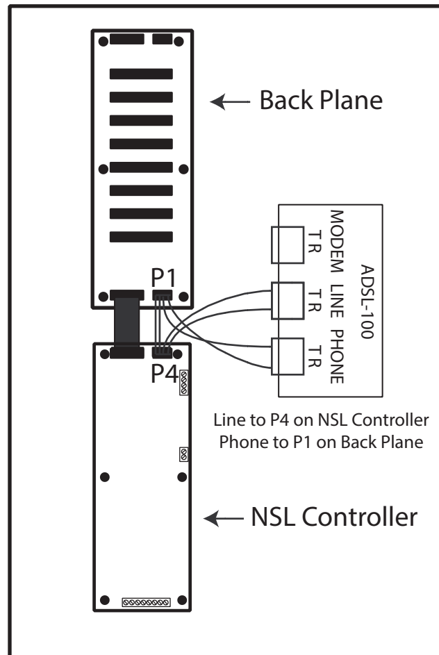
Figure 46. ADSL-100 Filter Module Installation
