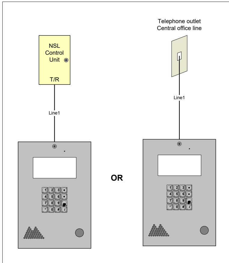
Figure 18. Single Lobby Control Unit
