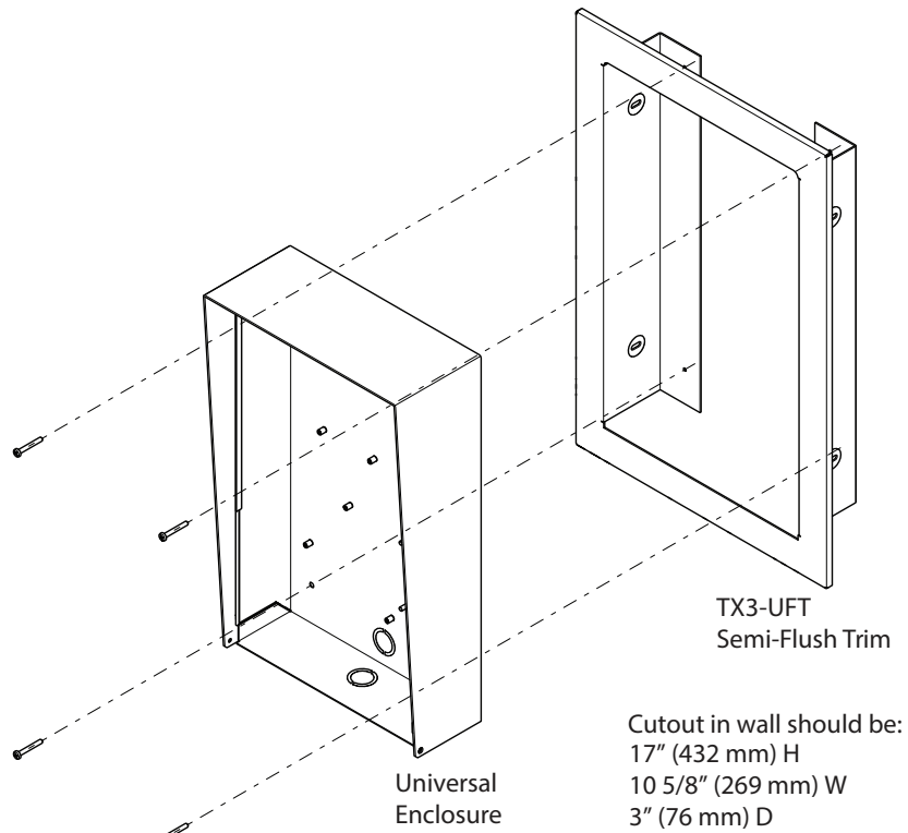
Figure 3 Mount TX3-UFT Universal Series Flush Trim Ring
