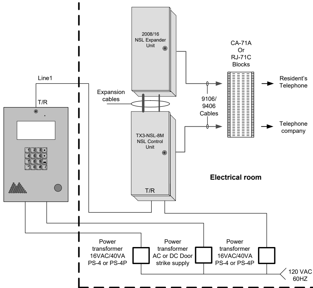
Figure 27. Lobby Control Unit Wiring
