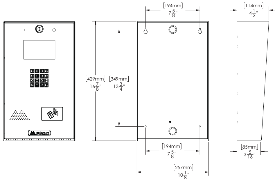
Figure 4 Dimensions of TX3-2000-8UR-C
