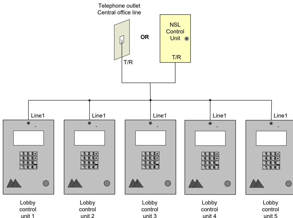
Figure 23. Many Lobby Control Units to One Line
