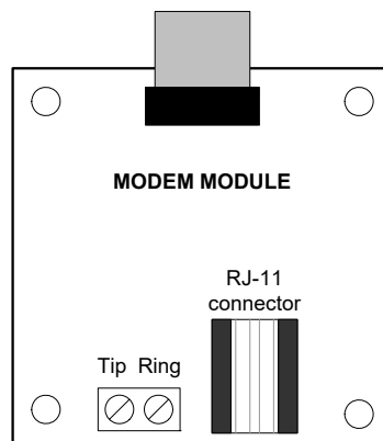
Figure 35. Modem Module Telephone Connectors
