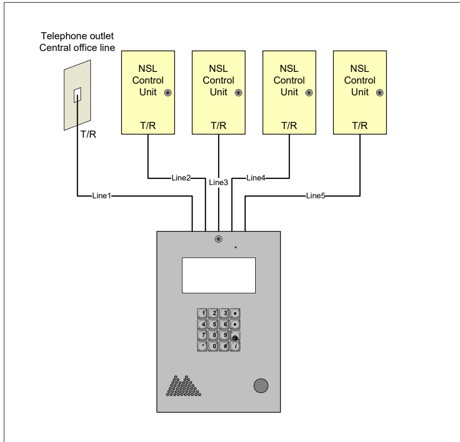
Figure 19. Single Lobby Control Unit with ADC and NSL Lines
