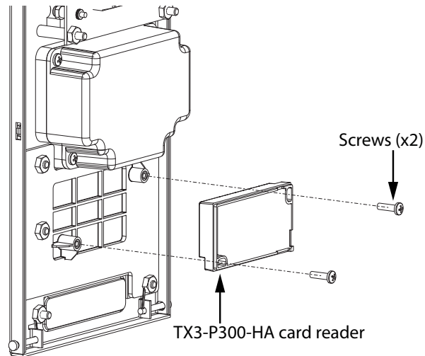
Figure 52. Install TX3-P300-HA
