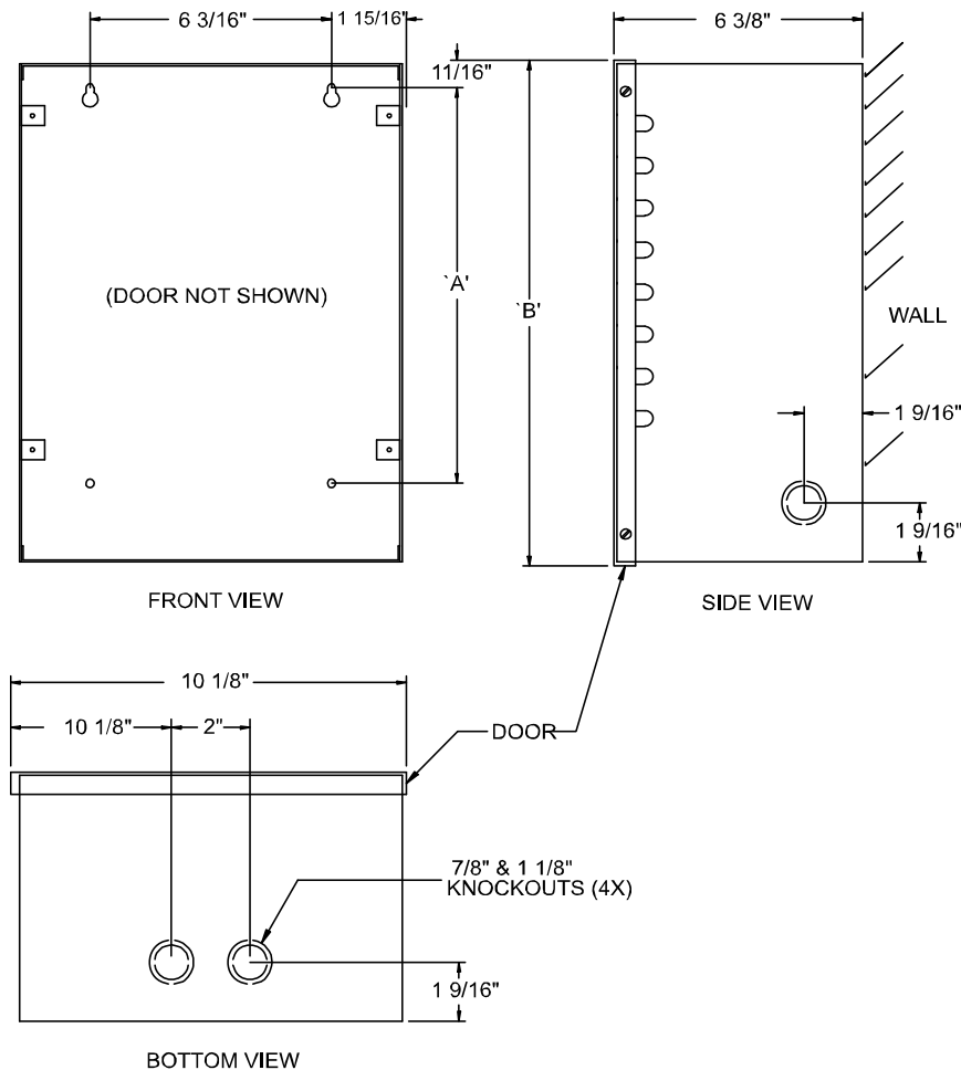
Figure 39. NSL Relay Cabinet
