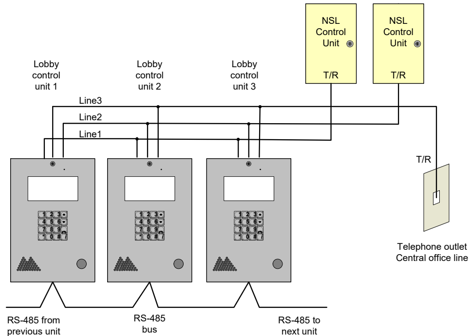
Figure 22. Multiple Lobby Control Units to Multiple Lines
