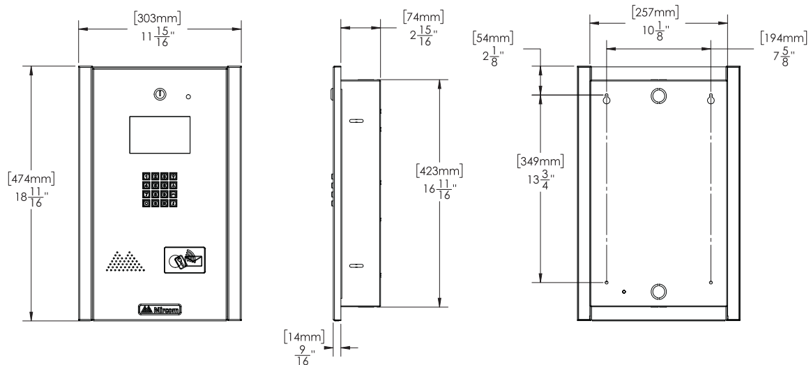
Figure 13 TX3-200-8C-C, TX3-1000-8C-C, TX3-2000-8C-C, TX3-120C-C Dimensions
