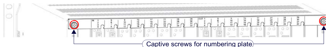
FIG. 1 Enova DGX 32/3200 only - Two captive screws hold numbering plate above boards
