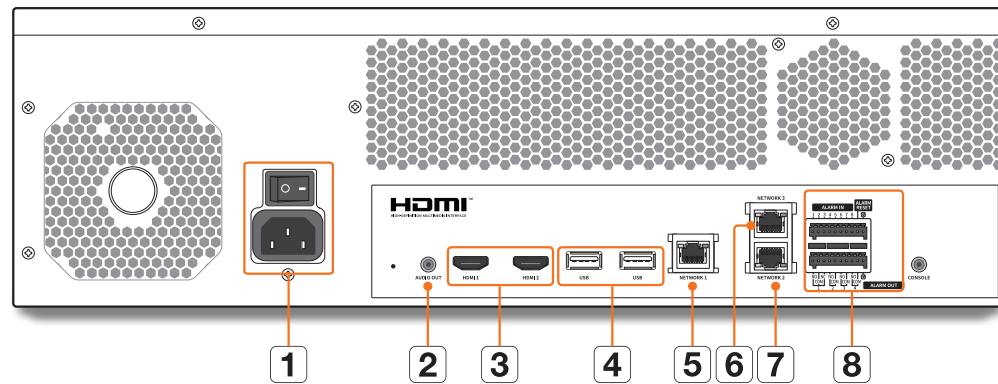
XRN-6420B4/XRN-3220B4
