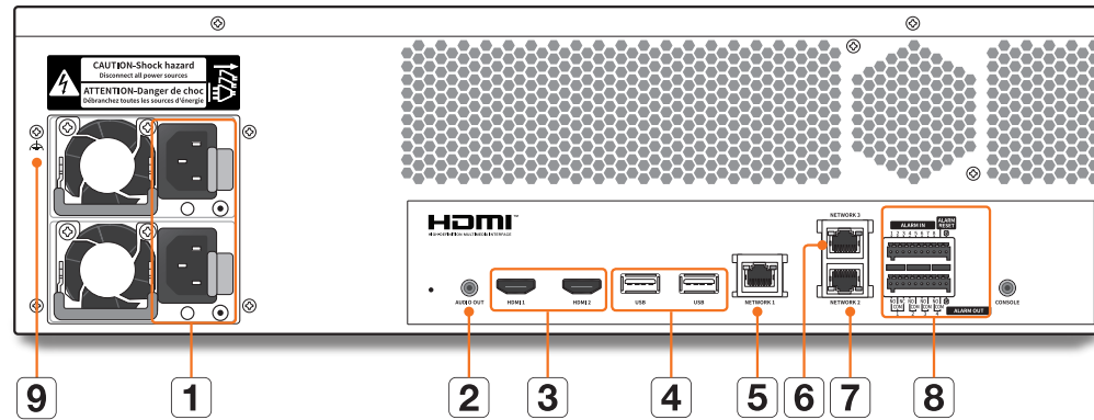
XRN-6420DB4
