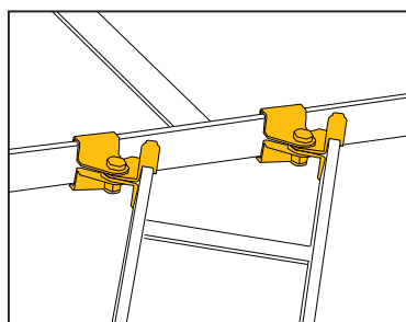
17 CLH-SKA adj. splice kit
