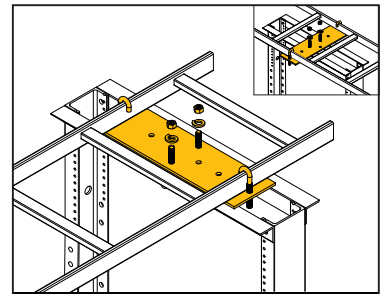
7 CLA-12RRP, CLA-18RRP relay rack plate kit
