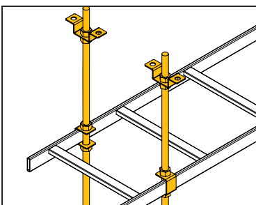
12 CLH-CK ceiling-mount kit
