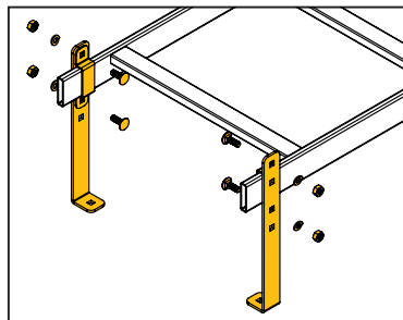
9 CLH-SK46 stand-off elevation kit
