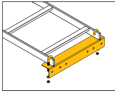
5 CLA-12WA, CLA-18WA wall angle bracket
