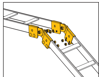
15 CLH-SKS swivel / adj. splice kit
