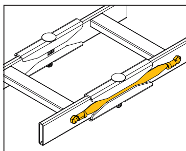
18 CLH-GSK grounding strap kit
