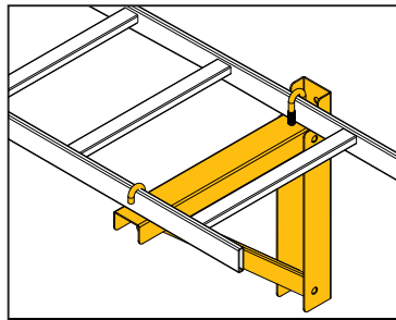
6 CLA-12WT, CLA-18WT wall triangle bracket
