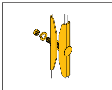
14 CLH-SKB butt splice kit
