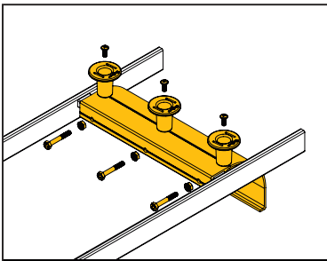
4 CLA-12RD, CLA-18RD cable radius drop
