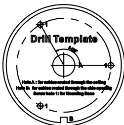
Figure 2-2 Drill Template
