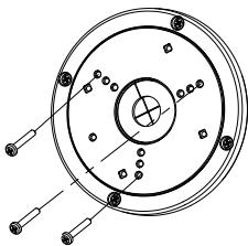
Figure 2-11 Install the Turret Camera's Mounting Base 5. Secure the junction box's body to the ceiling/wall with supplied screws.
