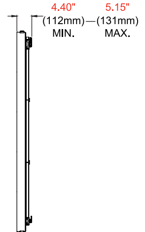
SIDE VIEW WITH MODULES
