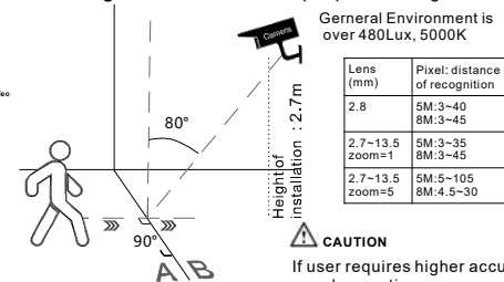
Figure 4-5 Installation of people counting
