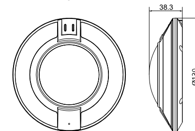
Figure 2-3 Dimensions (Unit:mm)
