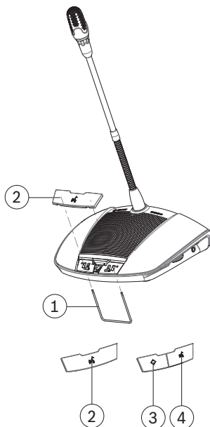
Figure 7.3: Exchanging the buttons
