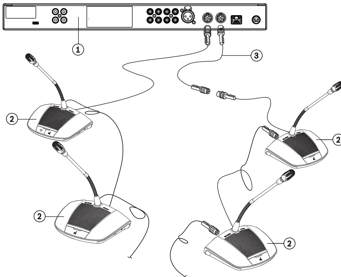
Figure 6.1: Connecting Discussion Devices
