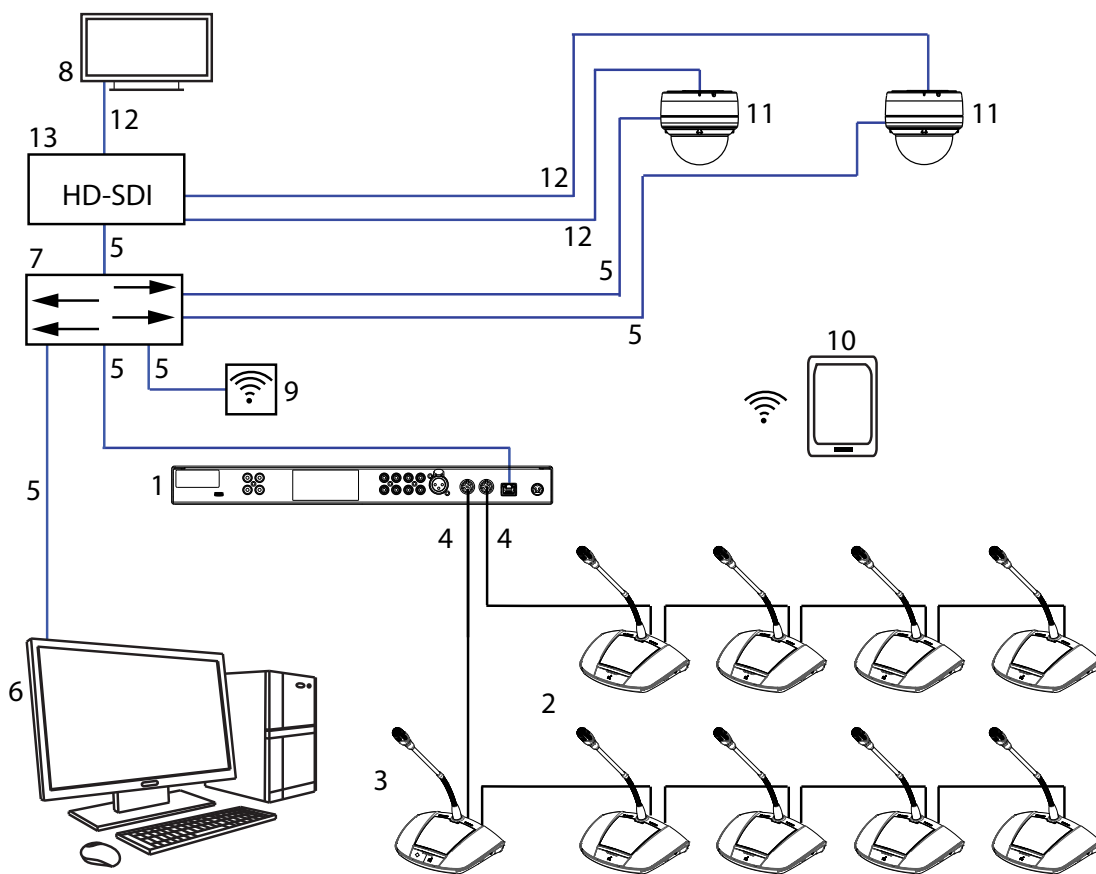
Figure 3.1: Typical system setup
