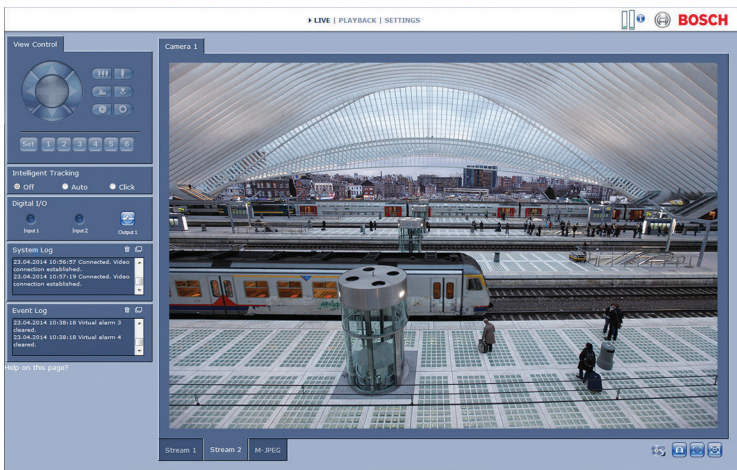
Figure 3.1: Live page
