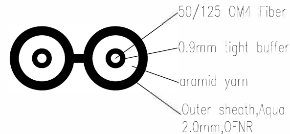
Ø2.0mm OFNR cable section
