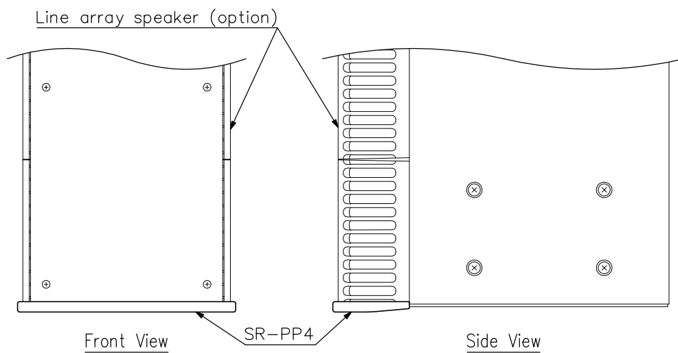
Mounting example (scale: 1/4)
