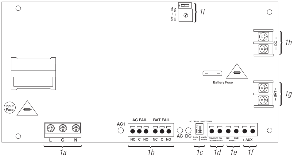
Fig. 1 - eFlowNBV configuration
