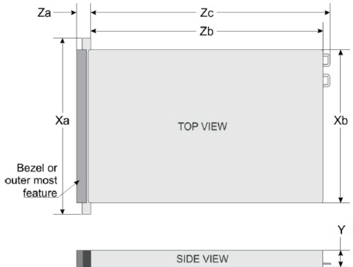
Chassis dimensions
