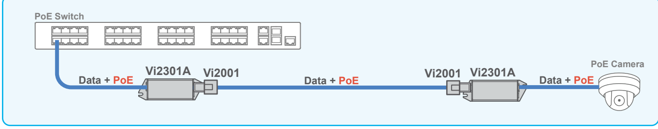
The Vi2001 can protect networking equipment against damaging voltage surges over extended UTP cables.
