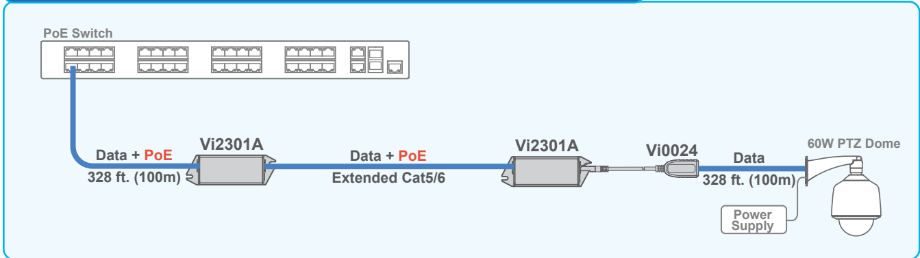
The Vi0024 can be used to power Ethernet Extenders using PoE when the end point is a Non PoE device.
