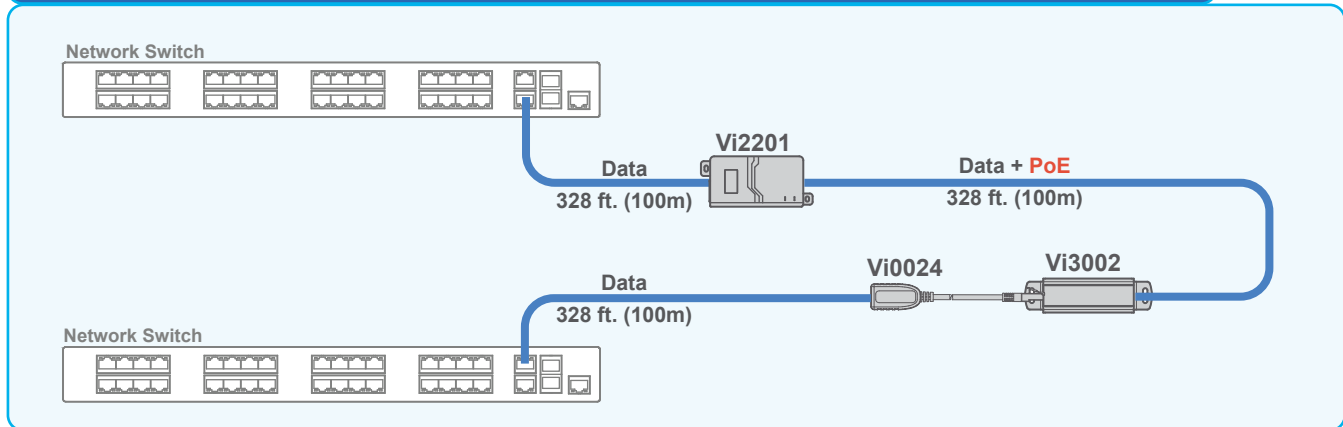
The Vi0024 can be used to power Ethernet Repeater with PoE when connecting non-PoE network switches.
