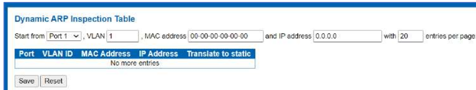
Figure 7–11-4: Dynamic ARP Inspection Table Screenshot
