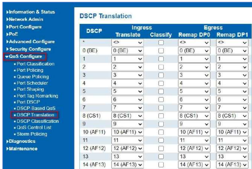
Figure 8-9 : DSCP Translation Page Screenshot
