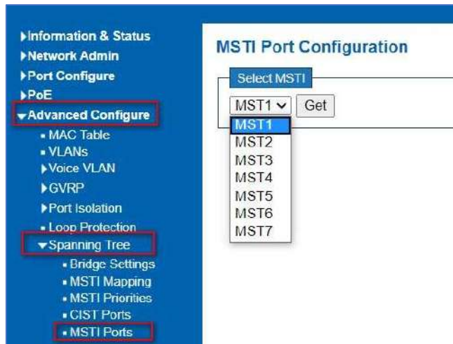
Figure 6-7.5 MSTI Port Configuration Page Screenshot
