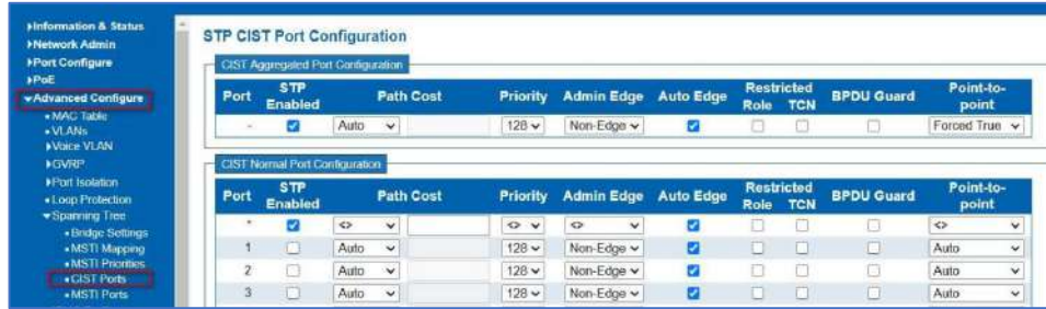
Figure 6-7.4 STP CIST Port Configuration Screenshot
