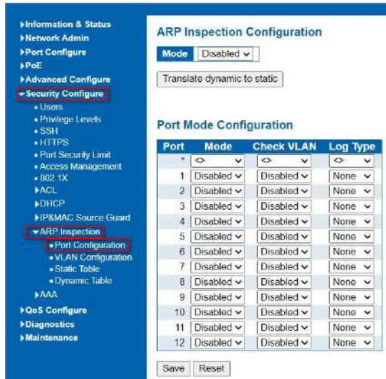
Figure 7-11-1 ARP Inspection Port Configuration Screen
