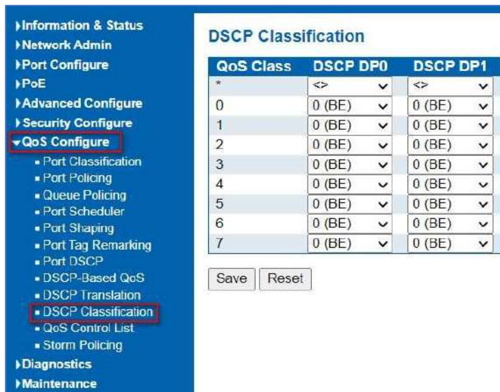
Figure 8-10: DSCP Classification Page Screenshot
