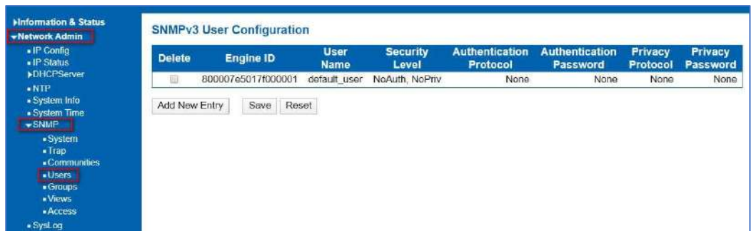
Figure 3-4.4 SNMP User Configuration Screen
