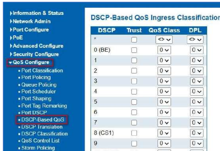
Figure 8-8: DSCP-based QoS Ingress Classification Page Screenshot
