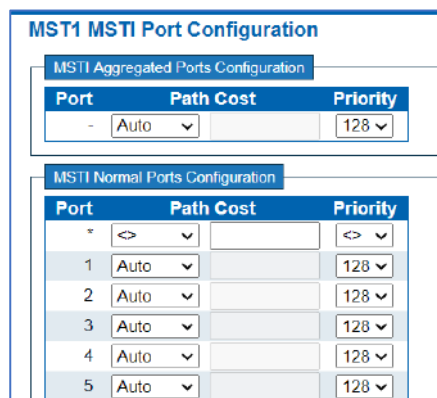
Figure 6-7.5 MST1 MSTI Port Configuration Page Screenshot
