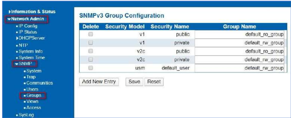
Figure 3-4.5 SNMP Group Configuration Screen
