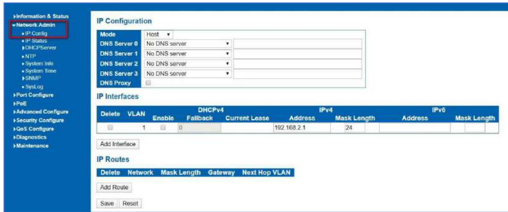
Figure 3-1 IP Configuration Screen
