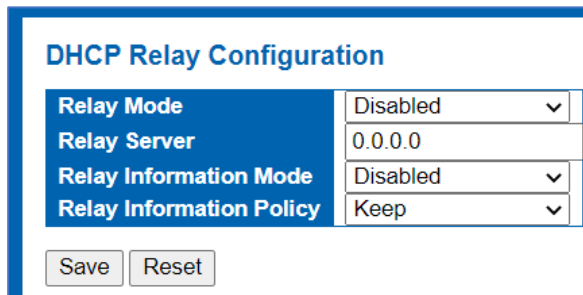
Figure 7-9-3-3 DHCP Relay Configuration Page Screenshot
