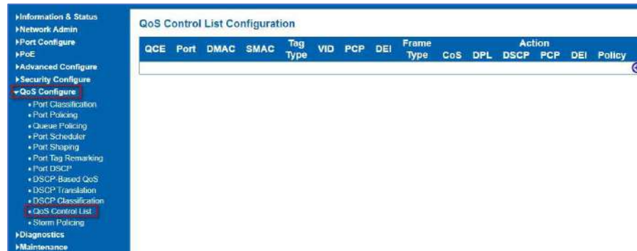
Figure 8-11: QoS Control List Configuration Page Screenshot
