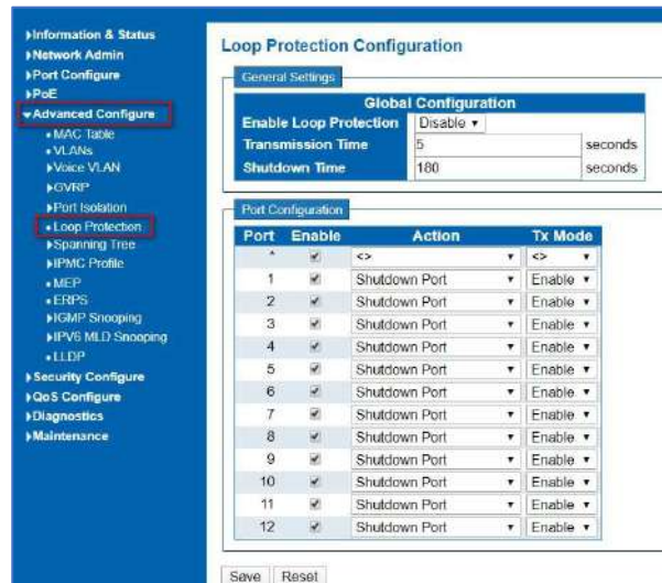
Figure 6-6 Loop Protection Configuration Screen
