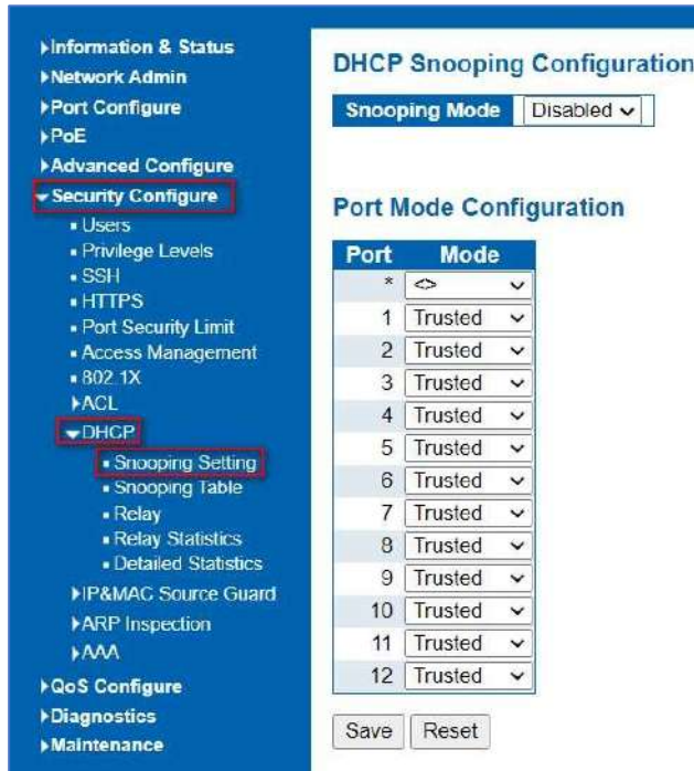
Figure 7-9-3-1 DHCP Snooping Configuration Screen
