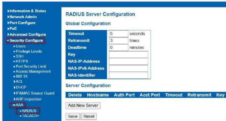
Figure 7-12-1: RADIUS Server Configuration Page Screenshot
