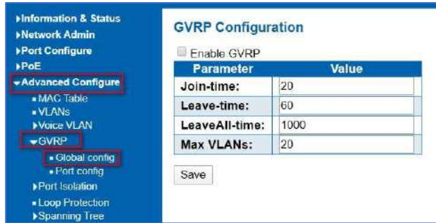
Figure 6-4 GVRP configuration screen
