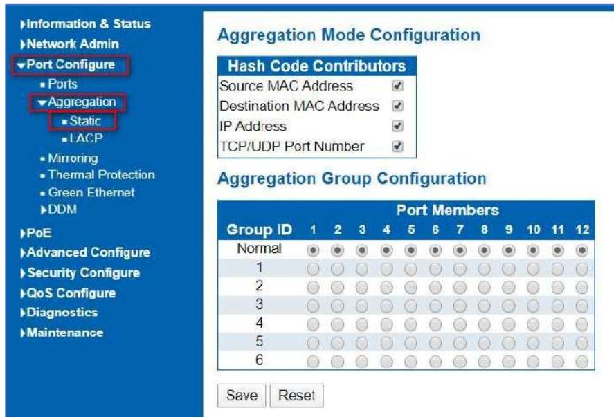
Figure 4-2.1 Port Static Aggregation Configuration Screen
