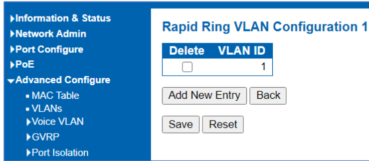
Figure 6-10-3 Rapid Ring VLAN Configuration Screen
