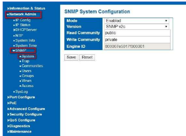
Figure 3-4.1 SNMP System Configuration Screen
