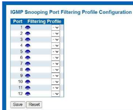
Figure 6-11-3: IGMP Snooping Port Filtering Profile Configuration Page Screenshot
