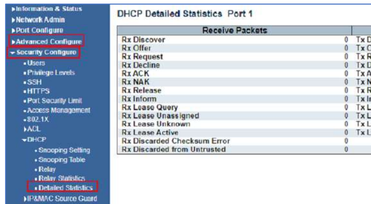
Figure 7-9-3-5: DHCP Detailed Statistics Screenshot
