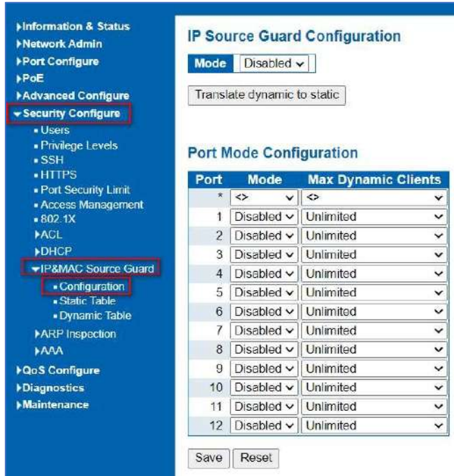
Figure 7-10-1 IP&MAC Guard-Port Configuration Screen
