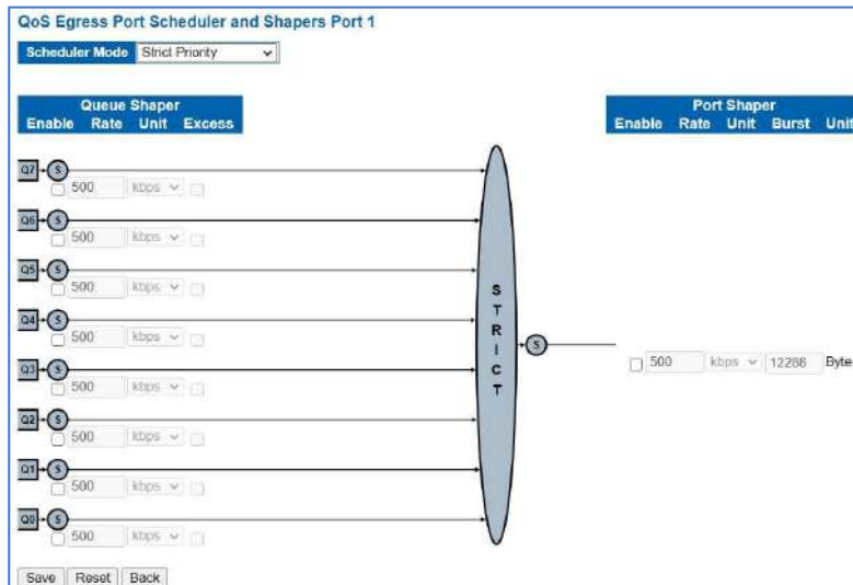
Figure 8-6/7: QoS Egress Port Schedule and Shapers Page Screenshot
