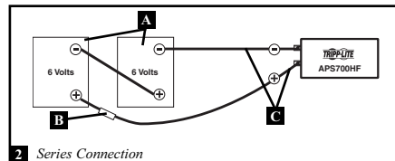
2 Series Connection
