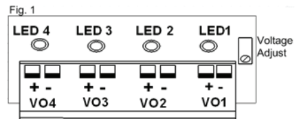
Power Module 2: Output Terminal Block for circuits 1-4 and Voltage
