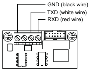
SA-232 Serial Port (RS-232), for connection to printers & computers, mounts in cabinet to base plate. Data Sheet S85005-0131 260097 Upload/download cable from SA-232 card to PC, DB9 to wire leads
