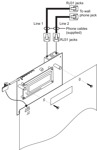
F-DACT Upload/download digital fire alarm (mounts in control panel) Data Sheet S85005-0126
