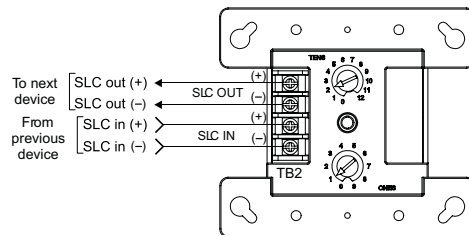
E-ISO SLC (Signalling Line Circuit) Fault Isolator Module (4 x 4 or two-gang standard mount) Data Sheet S85001-0611
