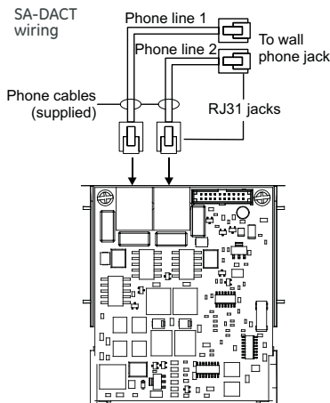
SA-DACT Dual Line Dialer/Modem, supports Contact ID, mounts in cabinet on base plate Data Sheet S85005-0131
