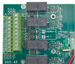
RDB4 distribution option board (for LP250 only)
