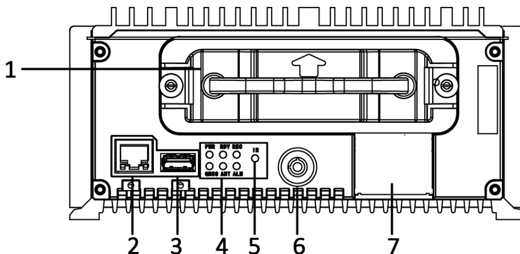
Figure 1-1 Front Panel
