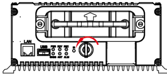
Figure 2-3 Unlock Dummy HDD
