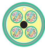
48 fibers
