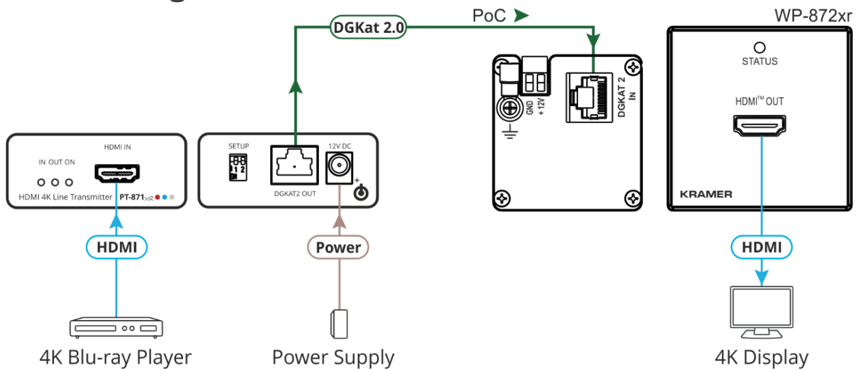
Figure 11: Connecting to PT-871xr and WP-872xr
