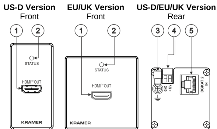
Figure 6: WP-872xr Line Receiver Wall-plate
