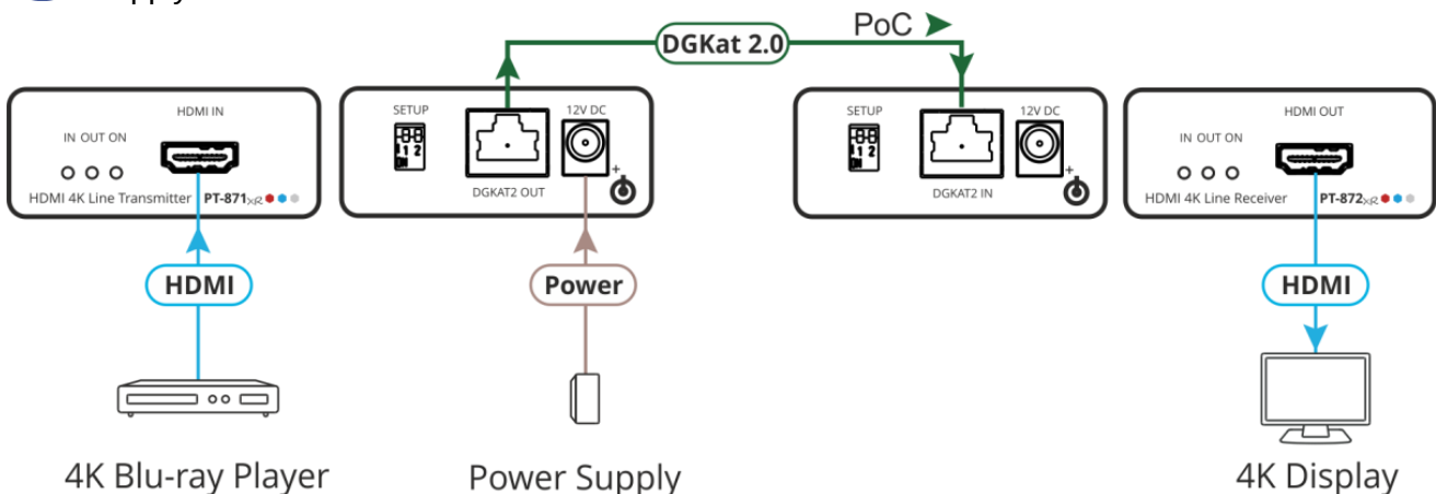
Figure 9: Connecting to PT-871/2xr-KIT
