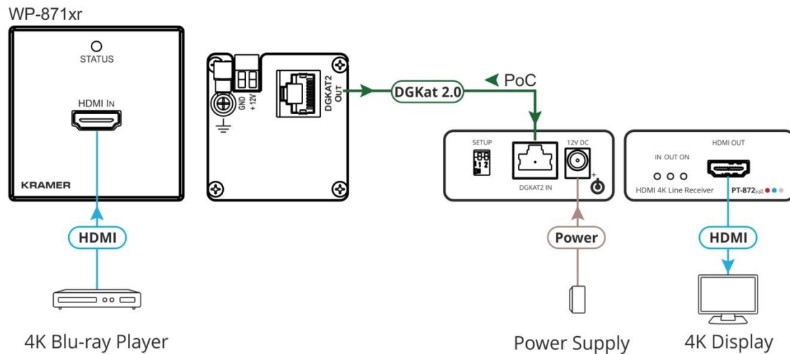
Figure 10: Connecting to WP-871xr and PT-872xr
