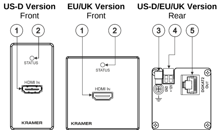
Figure 5: WP-871xr Line Transmitter Wall-plate
