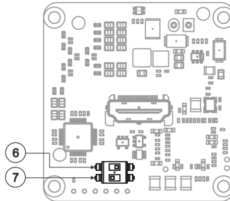
Figure 7: WP-871xr Line Transmitter Wall-plate – Front Panel Before Assembly
