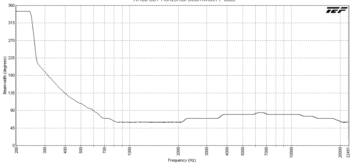
AH66-8ST Vertical Beamwidth (-6dB)
