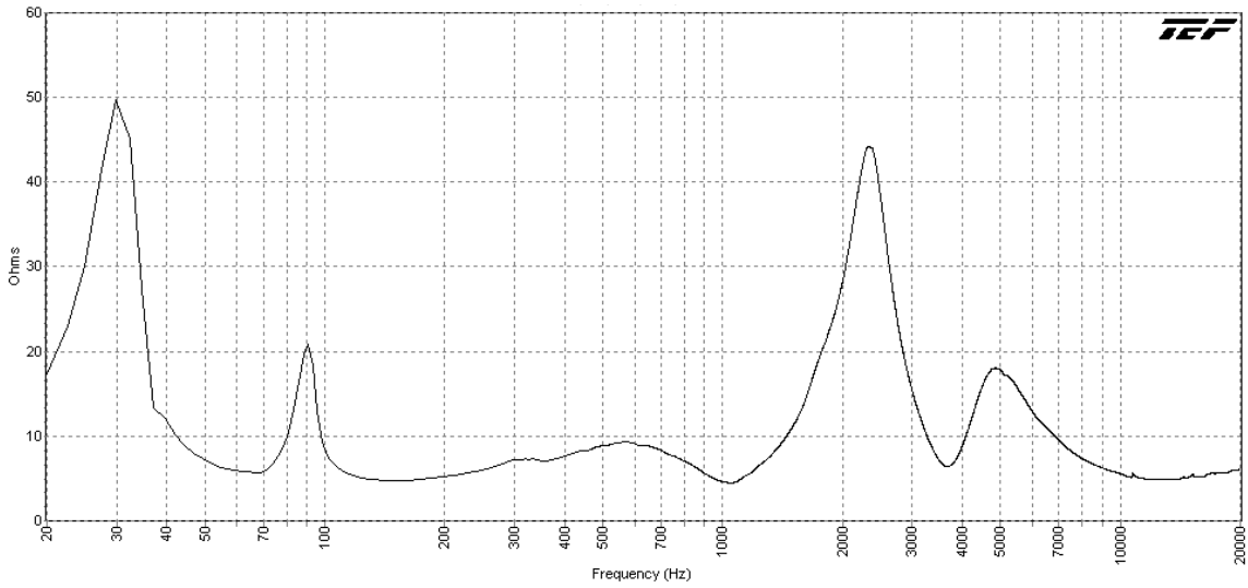
AH66-8ST Impedance (ohms) vs. Frequency
