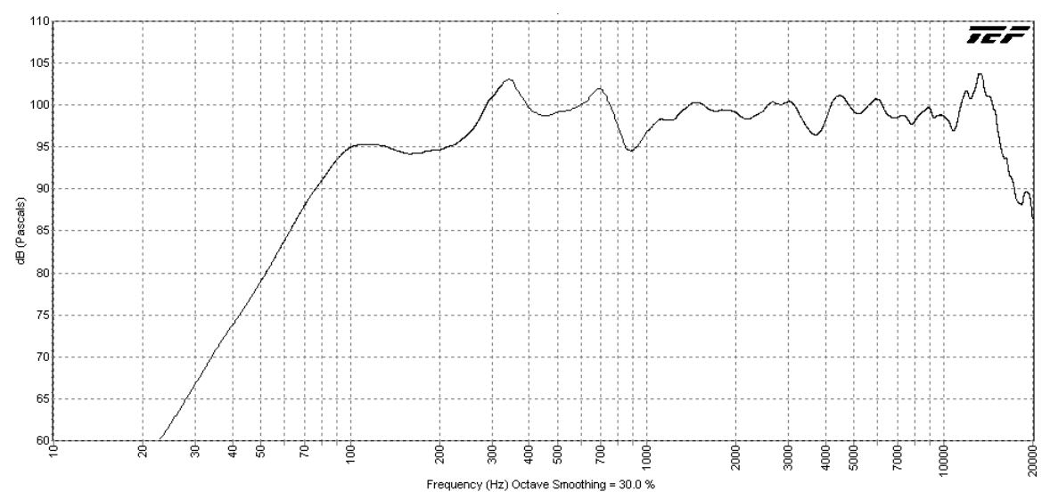
AH66-8ST Frequency Response
