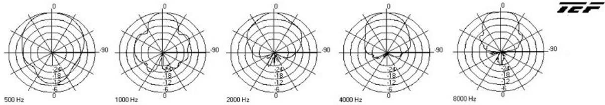
AH66-8ST Polars (Normalized To Zero On Axis) (-6dB)
