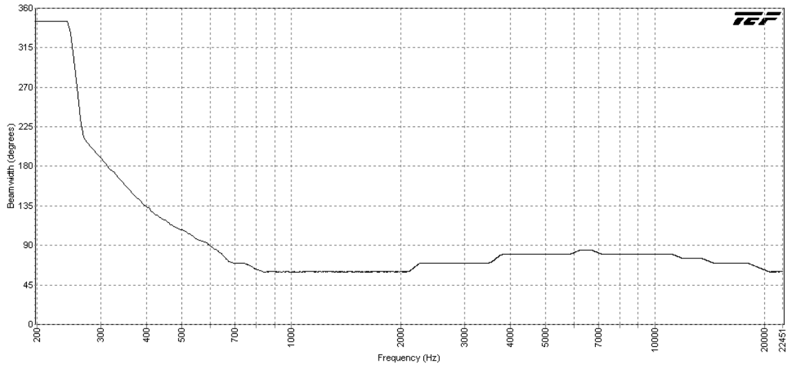
AH66-8ST Horizontal Beamwidth (-6dB)
