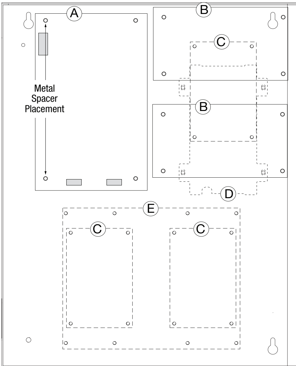
Fig. 2 - Altronix and Mercury configurations
