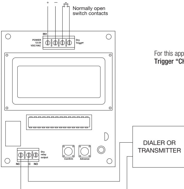
Fig. 2 - Guard Tour Supervisory Timer:
