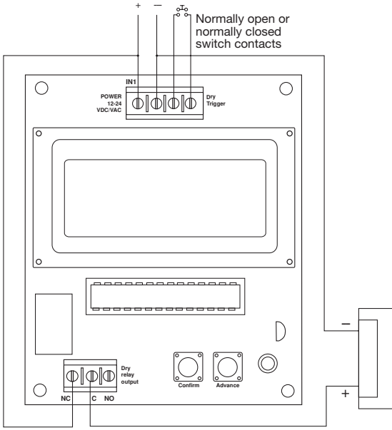
Fig. 7 - Delayed Egress:
