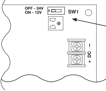
Fig. 1a - Maximal11 and Maximal33 Power Supply Board
