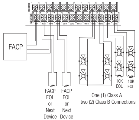
Fig. 7 Class B Input configuration and combination of Class A and Class B output configuration.
