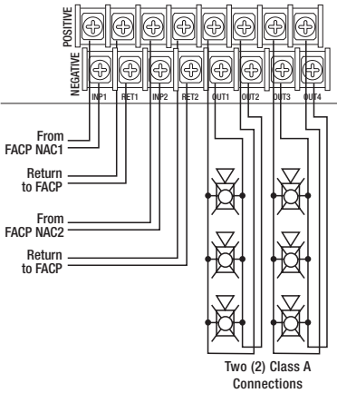
Fig. 6 Class A Configuration Inputs and Outputs
