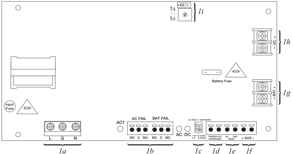
Fig. 1 - eFlowNB configuration
