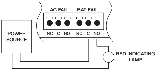
Fig. 3a - PD4UL Power Distribution Board
