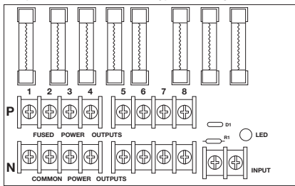
Fig. 3a - PD8UL Power Distribution Board Non Power-Limited Outputs
