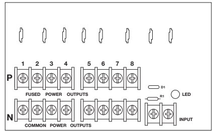
Fig. 3b - PD8ULCB - Power Distribution Board Class 2 Power-Limited Outputs
