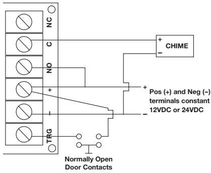
Fig. 1 - Timed Door Annunciator:
