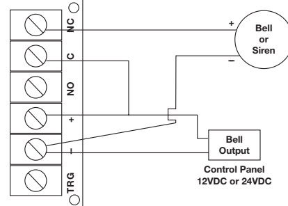
Fig. 7 - Bell Cut Off Timer:
