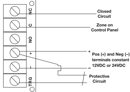
Fig. 3 - Swinger Eliminator:
