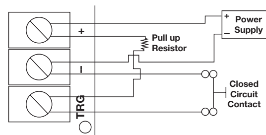
Fig. 8 - Closed Circuit Trigger Option:
