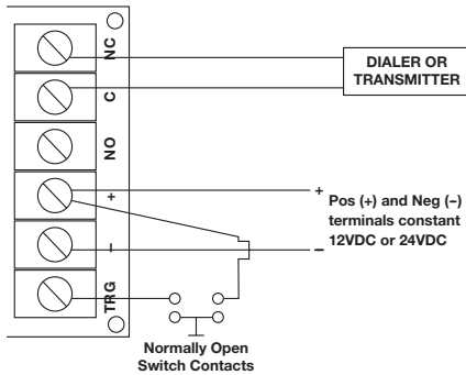
Fig. 2 - Guard Tour Supervisory Timer:
