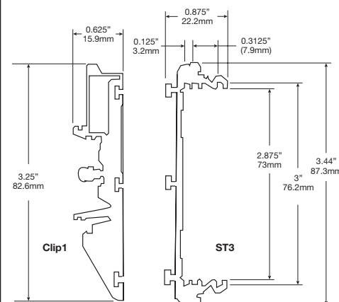
Fig. 1 - ST3 Mechanical Drawing
