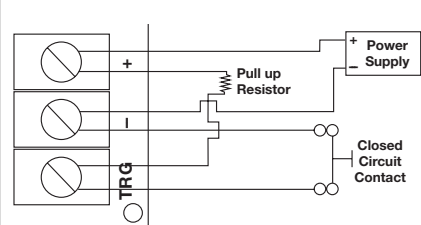
Fig. 8 - Closed Circuit Trigger Option:
