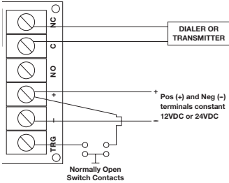
Fig. 2 - Guard Tour Supervisory Timer:
