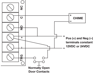
Fig. 1 - Timed Door Annunciator:
