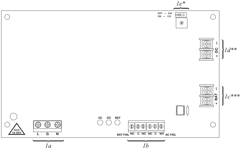
Fig. 1 - XBV configuration
