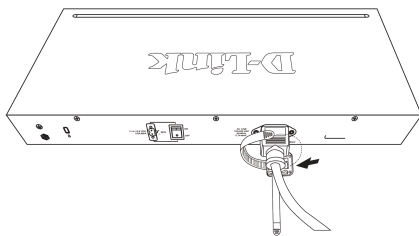
Wrap the retainer around the power cord
