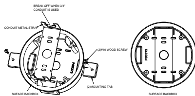
Figure 6: Surface Back box
