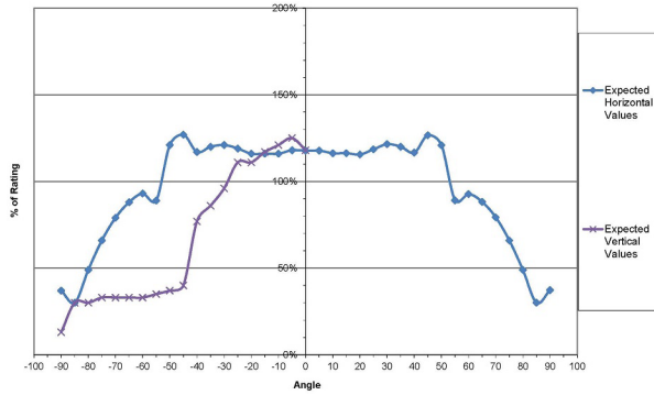
Figure 1: ELHSC/ELSTC/ELSTC-A Expected Light Output
